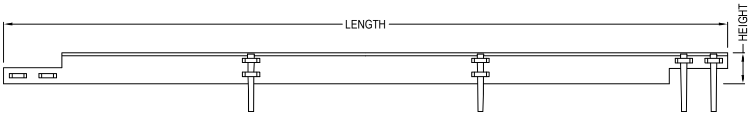
FRONT VIEW
